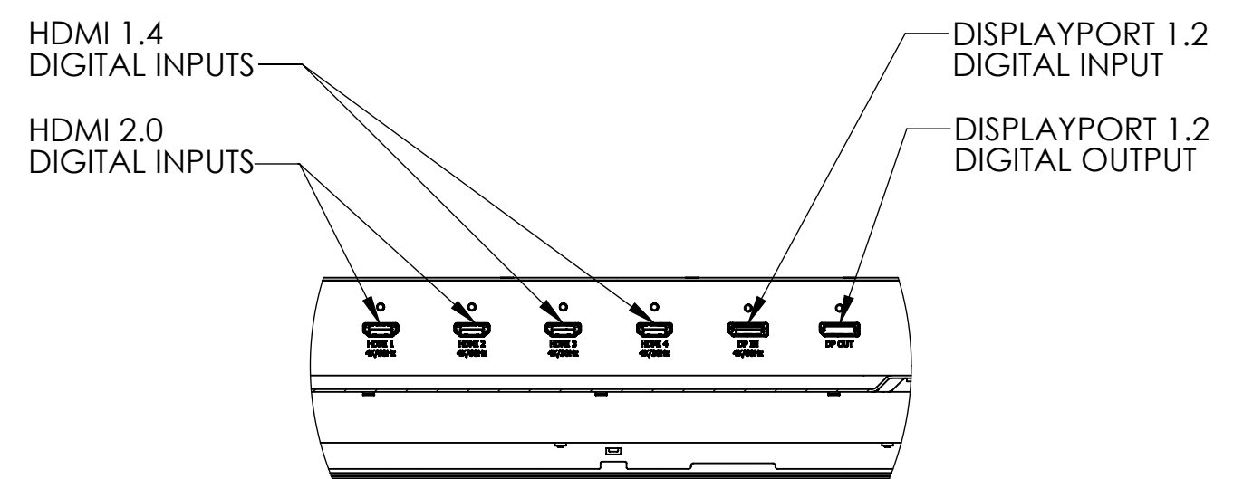
DETAIL B SCALE 1 : 3
